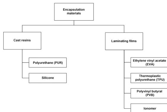
Figure 3: Classification of various potential encapsulation materials for PV modules
