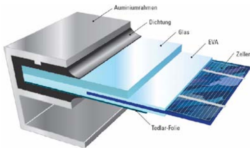
Figure 1: Basic design of a PV module [DGS - Berlin]
